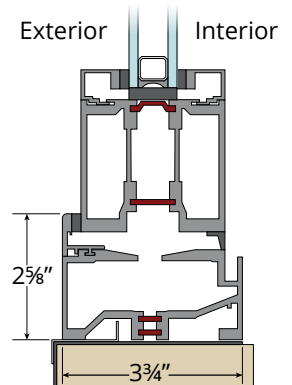
Extra High Performance Inswing Sill Not tested
