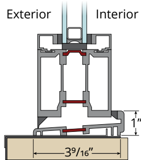
Standard Outswing Sill 6PSF lab water performance 4PSF field water performance
