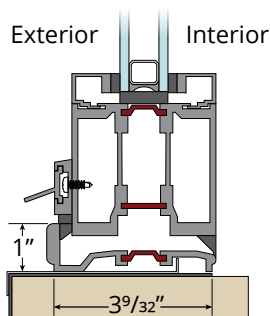
Standard Inswing Sill Not tested
