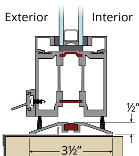
ADA Sill Limited/no water performance ADA compliant
