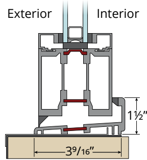
High Performance Outswing Sill 6PSF lab water performance 4PSF field water performance
