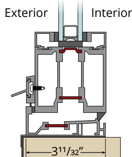
High Performance Inswing Sill Not tested
