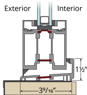
High Performance Outswing Sill 10PSF lab water performance 6.67PSF field water performance
