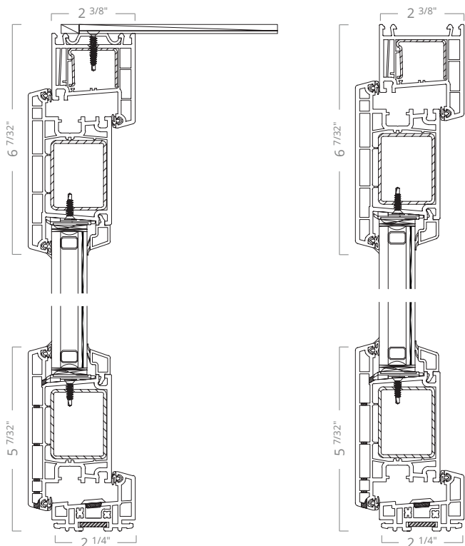
Terrace Door w/ Flange
