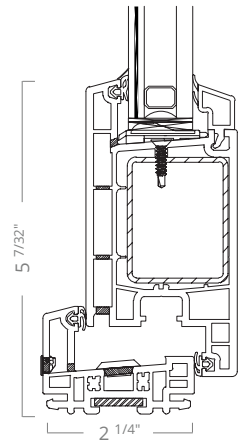
InSwing Sill
