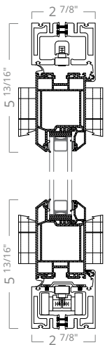
Head & Sill
