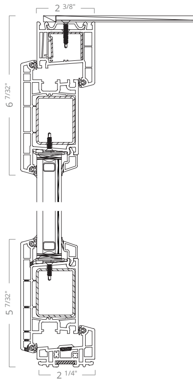
Terrace Door w/ Flange
