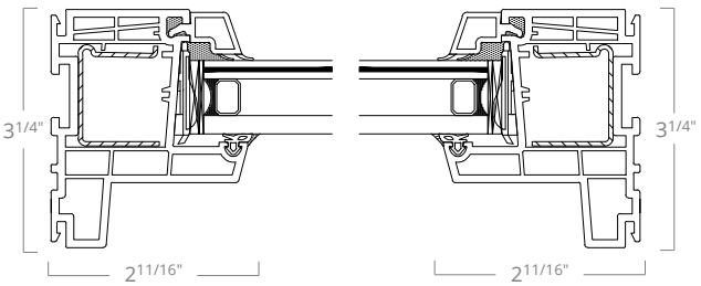
North American w/o Flange Jamb Details
