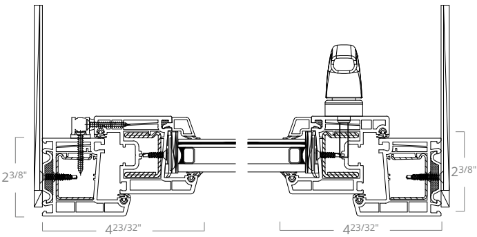
European w/Flange Jamb Details
