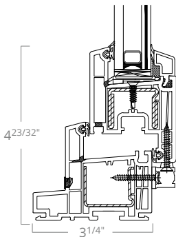
North American w/o Flange Head & Sill Details
