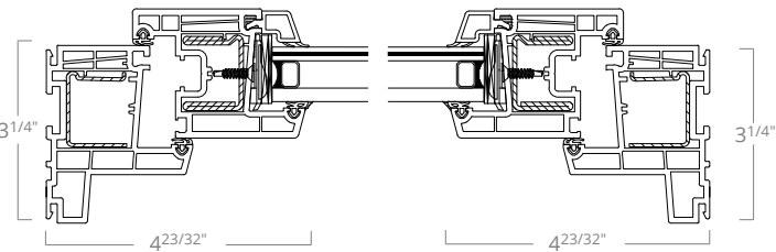
North American w/o Flange Jamb Details
