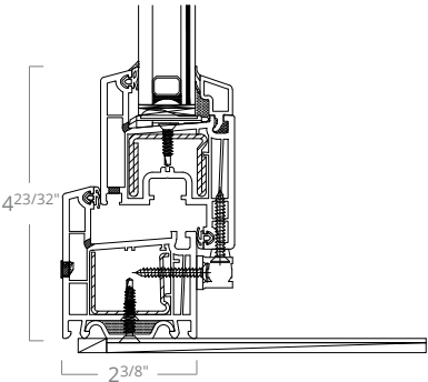
European w/ Flange Head & Sill Details
