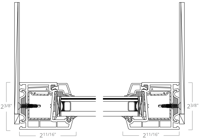
European w/Flange Jamb Details
