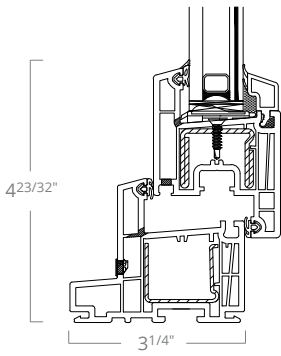
North American w/o Flange Head & Sill Details
