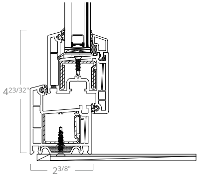
European w/ Flange Head & Sill Details
