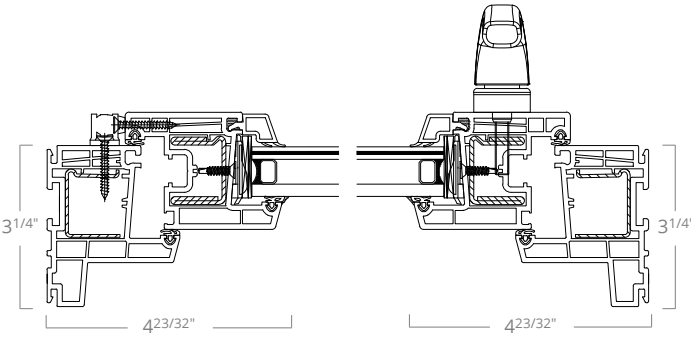
North American w/o Flange Jamb Details
