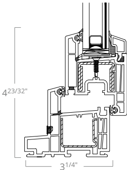
North American w/o Flange Head & Sill Details
