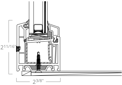
European w/ Flange Head & Sill Details
