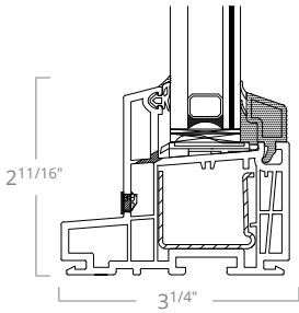
North American w/o Flange Head & Sill Details
