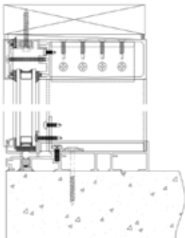
Heavy Glazing Bar
