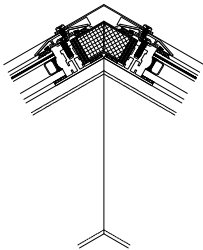
Double Pitch Ridge Detail
