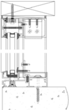
Regular Glazing Bar
