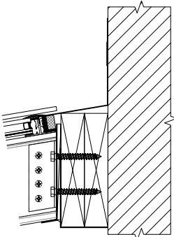
Lean-To Ridge Detail
