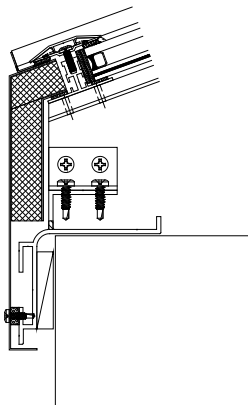
VARIABLE PITCH WELDED CURB
