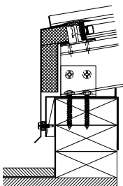
PAN FLASHING SILL
