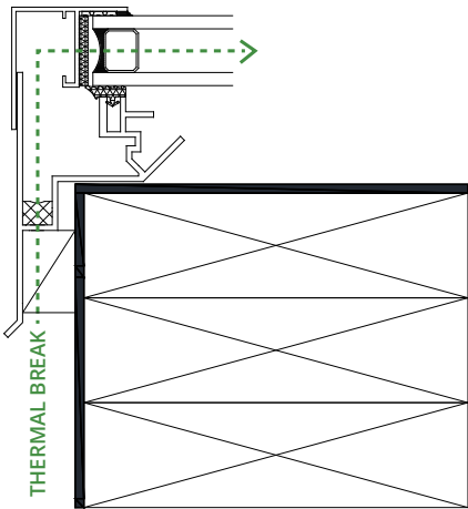
G2 FLAT WELDED CURB
