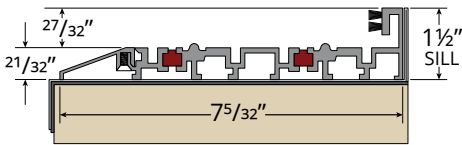
G3 Lift-Slide Thermal Sill — 1 1/2" Up Leg 8PSF expected field water performance
