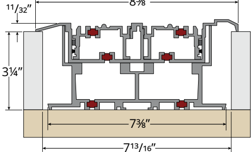
ADA Tank Sill 12PSF expected field water performance Can use exterior weep flaps or drain tubes ADA compliant
