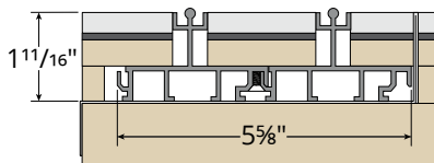
G3 Sliding Non-Thermal Tile Sill 5.2PSF expected field water performance Sill pan required for water performance ADA compliant
