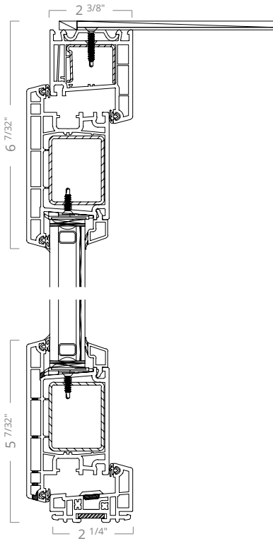
Terrace Door w/ Flange
