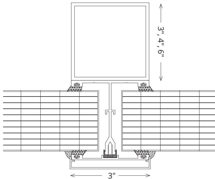
Wall Intermediary
